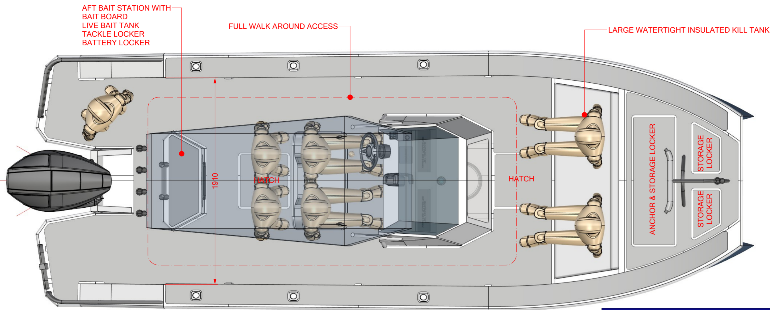
PLAN VIEW
